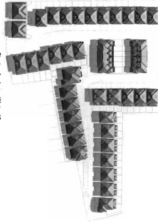
Shadow Analysis - Winter 12pm
